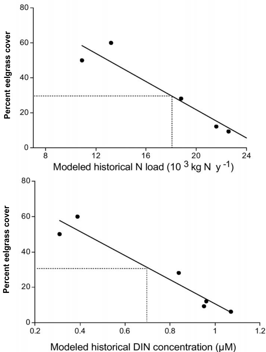
Figure 7-1. Relationship between nitrogen (N) loads, dissolved inorganic nitrogen (DIN) concentration, and percent eelgrass cover. Top: nitrogen loading model estimates of N loads from 1938 to the present plotted against percent eelgrass cover in Waquoit Bay in the corresponding years. To restore eelgrass in Waquoit Bay to 30% of the original area it is necessary to reduce the N Load to 18,000 kg N/yr. Bottom: estuarine loading model-predicted N concentrations in Waquoit Bay since 1938 plotted against eelgrass area. To restore eelgrass in Waquoit Bay to 30% of the original area would require attaining a dissolved inorganic concentration of about 0.75 μM.
