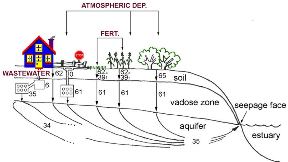
Figure 5-1. Schematic of the nitrogen loading model. Inputs of wastewater-, fertilizer-, and atmospherically derived nitrogen to the watershed and the percent losses (shown as numbers) as the nitrogen from the three main sources percolates through the watershed and enters the estuary at the seepage face.
