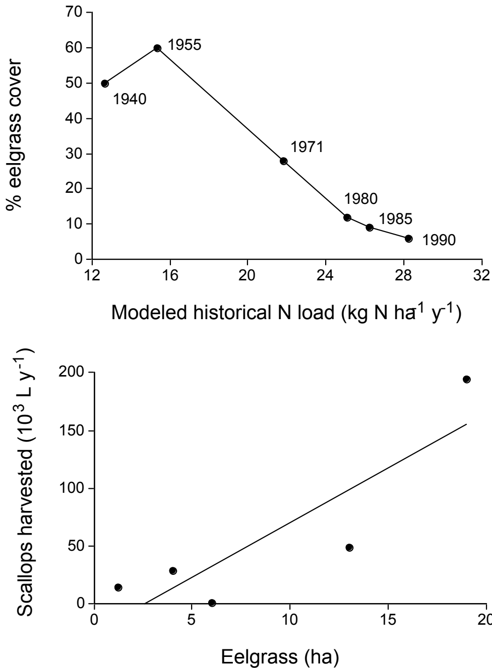
Figure 6-3. Decreases in area of eelgrass and volume of scallops harvested over time as a function of increasing nitrogen (N) loads. Top: percent of area covered with eelgrass in Waquoit Bay estimated by aerial photographs between 1940 and 1990 (Costa 1988, Short and Burdick 1996) plotted against modeled historical N loads. Bottom: the number of reported scallops harvested in Waquoit Bay as a function of eelgrass area. Scallop data are from the Shellfish Warden's annual reports, in the Town of Falmouth Annual Report.
