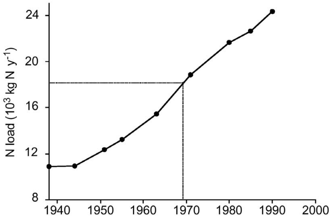
Figure 7-2. Historical changes in nitrogen (N) loading predicted by the nitrogen loading model. If the management target is a return to 30% eelgrass cover, then managers must reduce N loads to 18,000 kg N/yr, loads that are comparable to those of around 1970.
